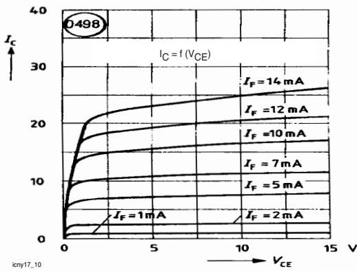
Figure 10. Output Characteristics
